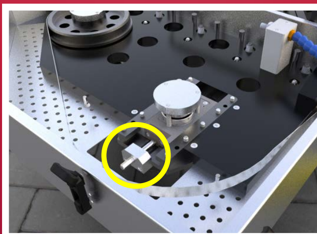
BLADE TENSION ADJUSTMENT
